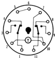
OFF DELAY
