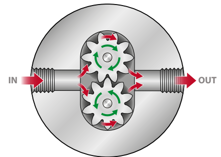
Operating principle
