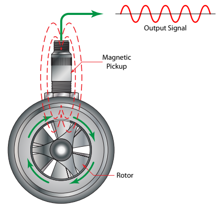
Illustration of electric signal generated by rotor movement
